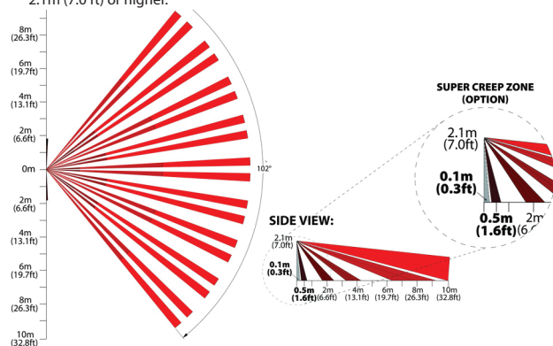
Figure 2: Beam Pattern
