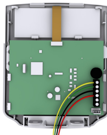
Figure 4: Wiring
